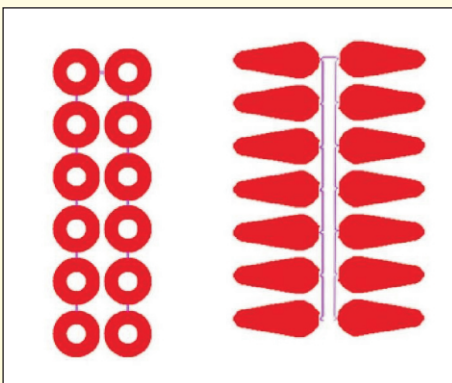
Bridge Cut
